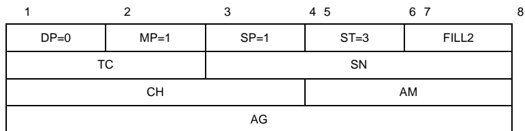
Figure 5-9. CLEAR CONFIRMATION by ADLP packet
