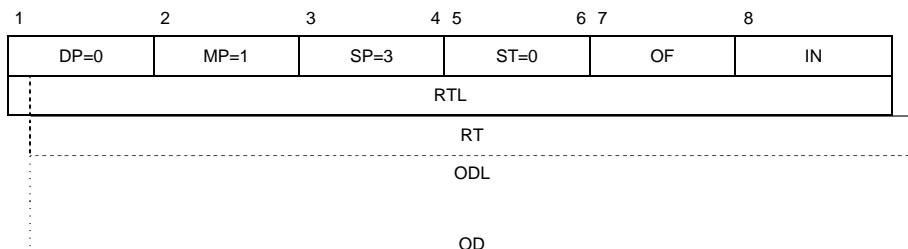
Figure 5-19. ROUTE packet
