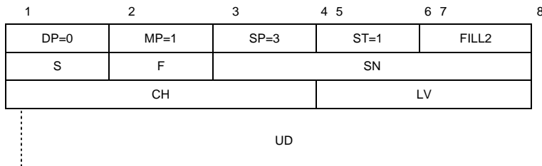
Figure 5-12. INTERRUPT packet
