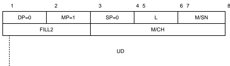
Figure 5-22. LONG FORM MSP packet
