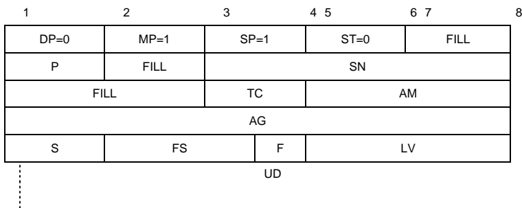
Figure 5-4. CALL REQUEST by GDLP packet
