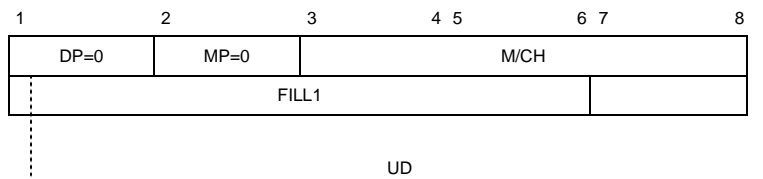
Figure 5-21. SHORT FORM MSP packet
