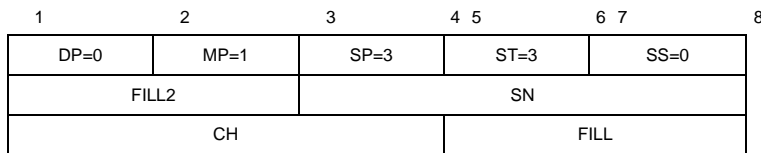
Figure 5-13. INTERRUPT CONFIRMATION packet
