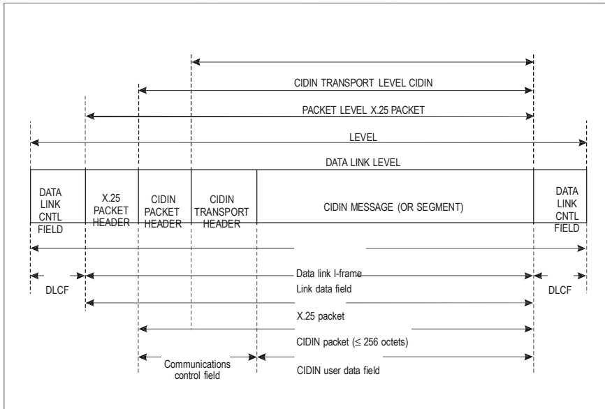
Figure 8-2. CIDIN terminology
