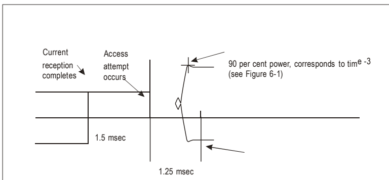
Figure 6-3. Receive to Transmit turnaround time
