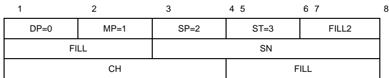
Figure 5-18. RESET CONFIRMATION packet
