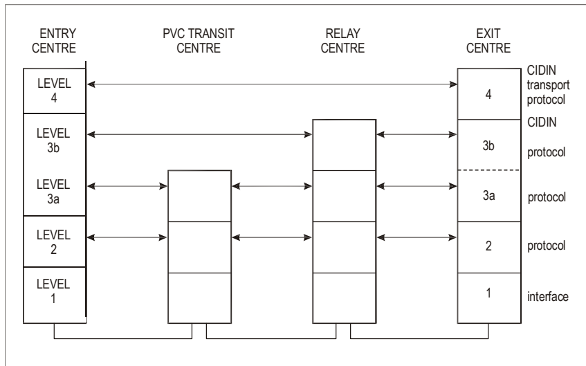
Figure 8-1. CIDIN protocol levels
