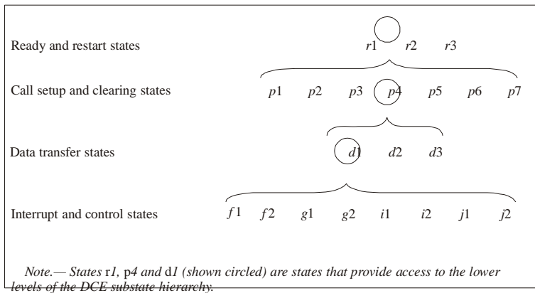
Figure 5-2. DCE substate hierarchy
