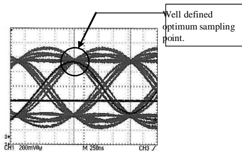
Figure 12-3. Ideal eye diagram
