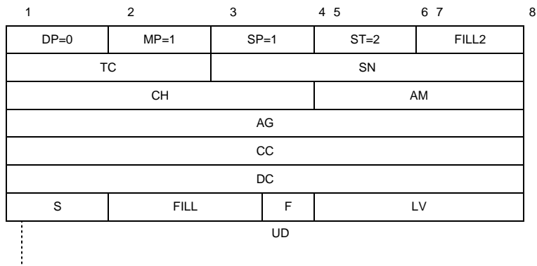
Figure 5-7. CLEAR REQUEST by ADLP packet
