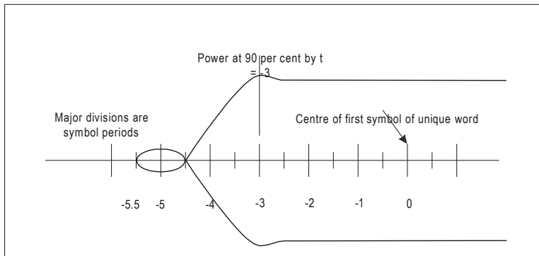
Figure 6-1. Transmitter power stabilization
