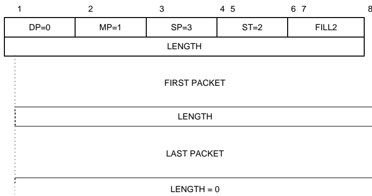
Figure 5-20. MULTIPLEX packet
