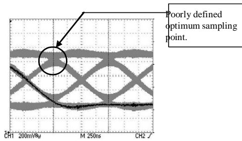
Figure 12-4. Distorted eye diagram
