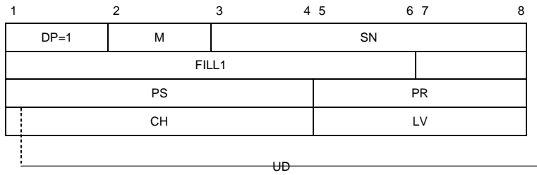
Figure 5-11. DATA packet
