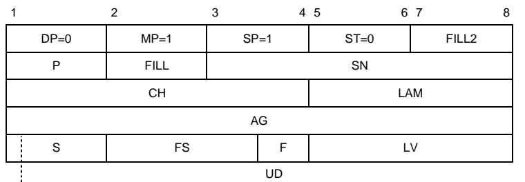
Figure 5-3. CALL REQUEST by ADLP packet
