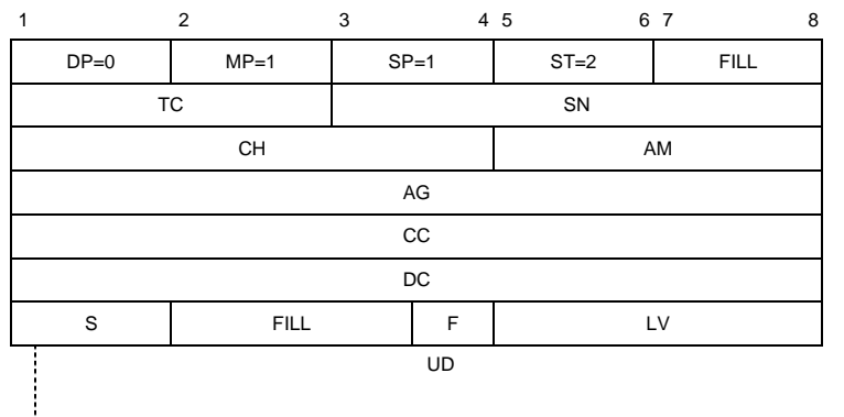
Figure 5-8. CLEAR REQUEST by GDLP packet
