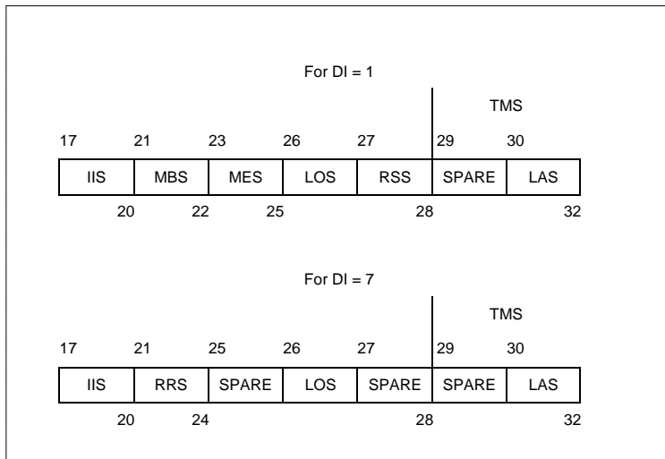
Figure 5-1. The SD field structure
