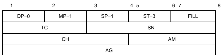
Figure 5-10. CLEAR CONFIRMATION by GDLP packet
