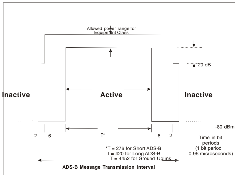
Figure 12-2. Time/amplitude profile of UAT message transmission
