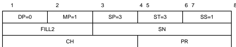
Figure 5-14. REJECT packet
