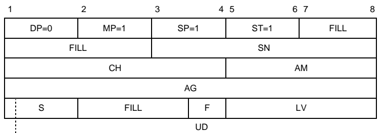
Figure 5-6. CALL ACCEPT by GDLP packet
