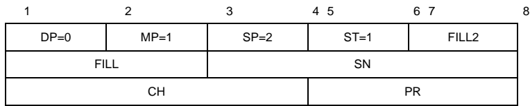
Figure 5-16. RECEIVE NOT READY packet
