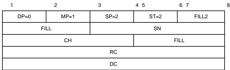
Figure 5-17. RESET REQUEST packet
