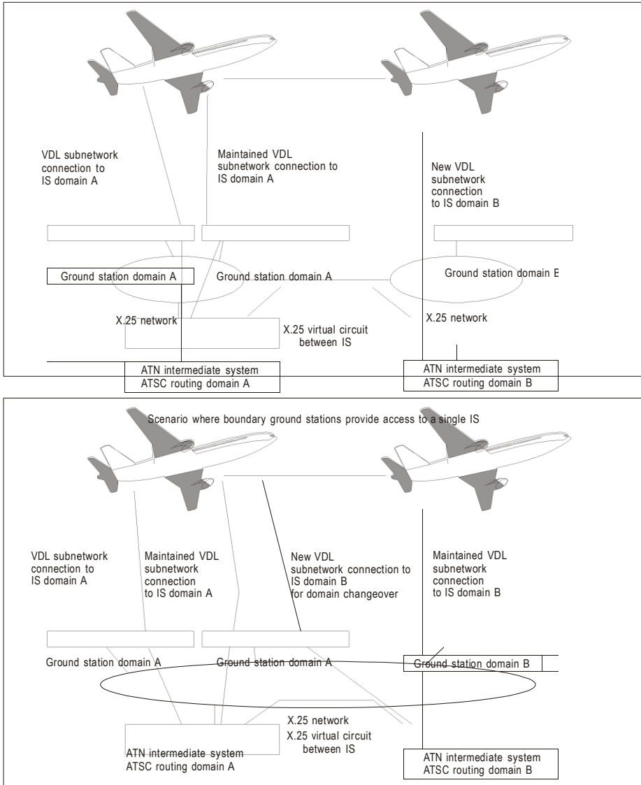
Scenario where boundary ground stations provide access to IS in two routing domains
