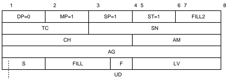
Figure 5-5. CALL ACCEPT by ADLP packet
