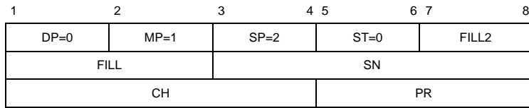
Figure 5-15. RECEIVE READY packet
