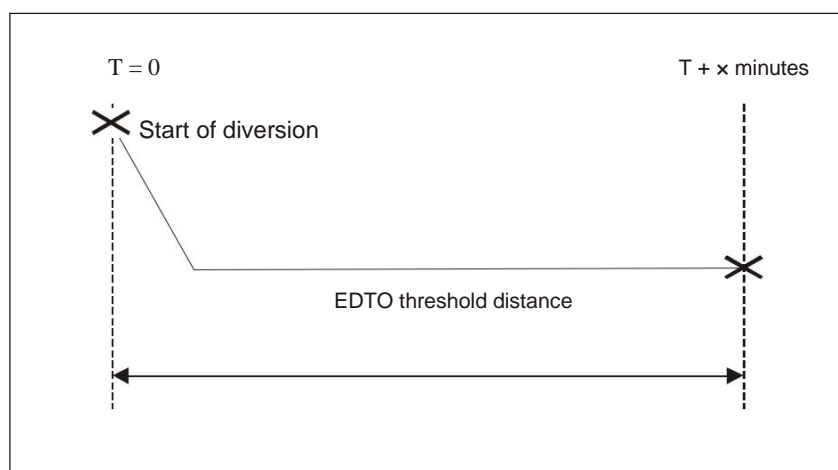
Figure C-8. Threshold distance — aeroplanes with two turbine engines
